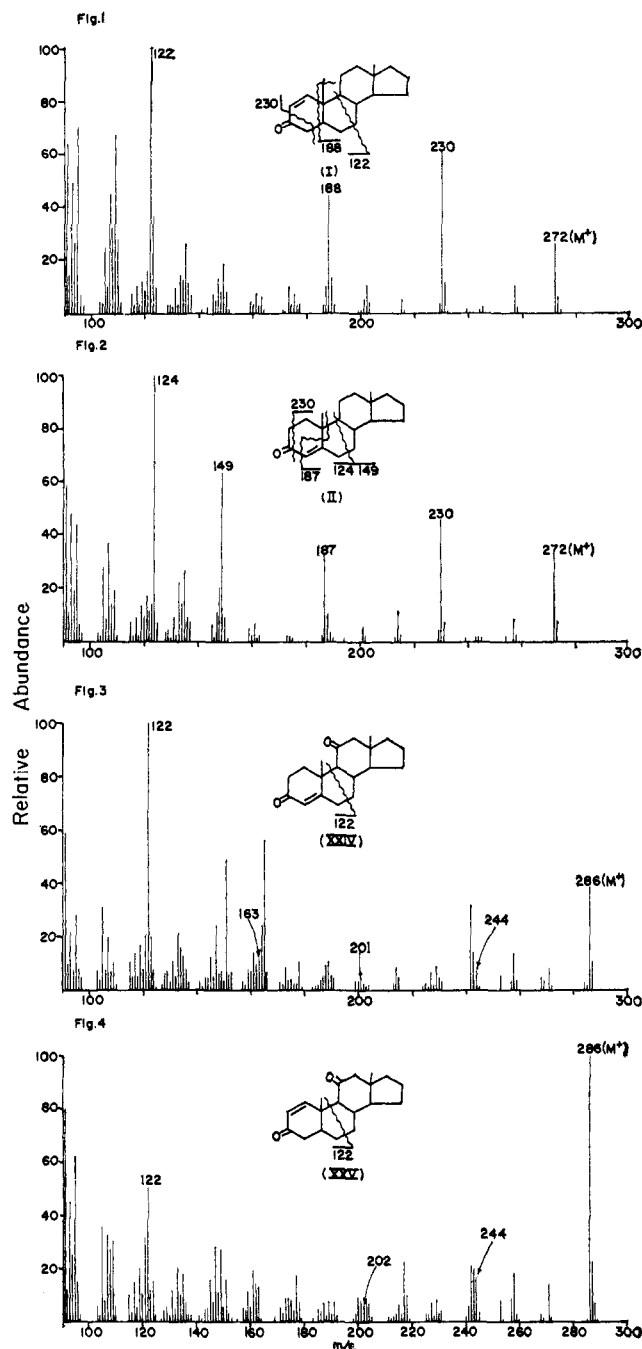
Fig. 1.—Mass spectrum of \Delta^1 -5 \alpha -androst-3-one.
